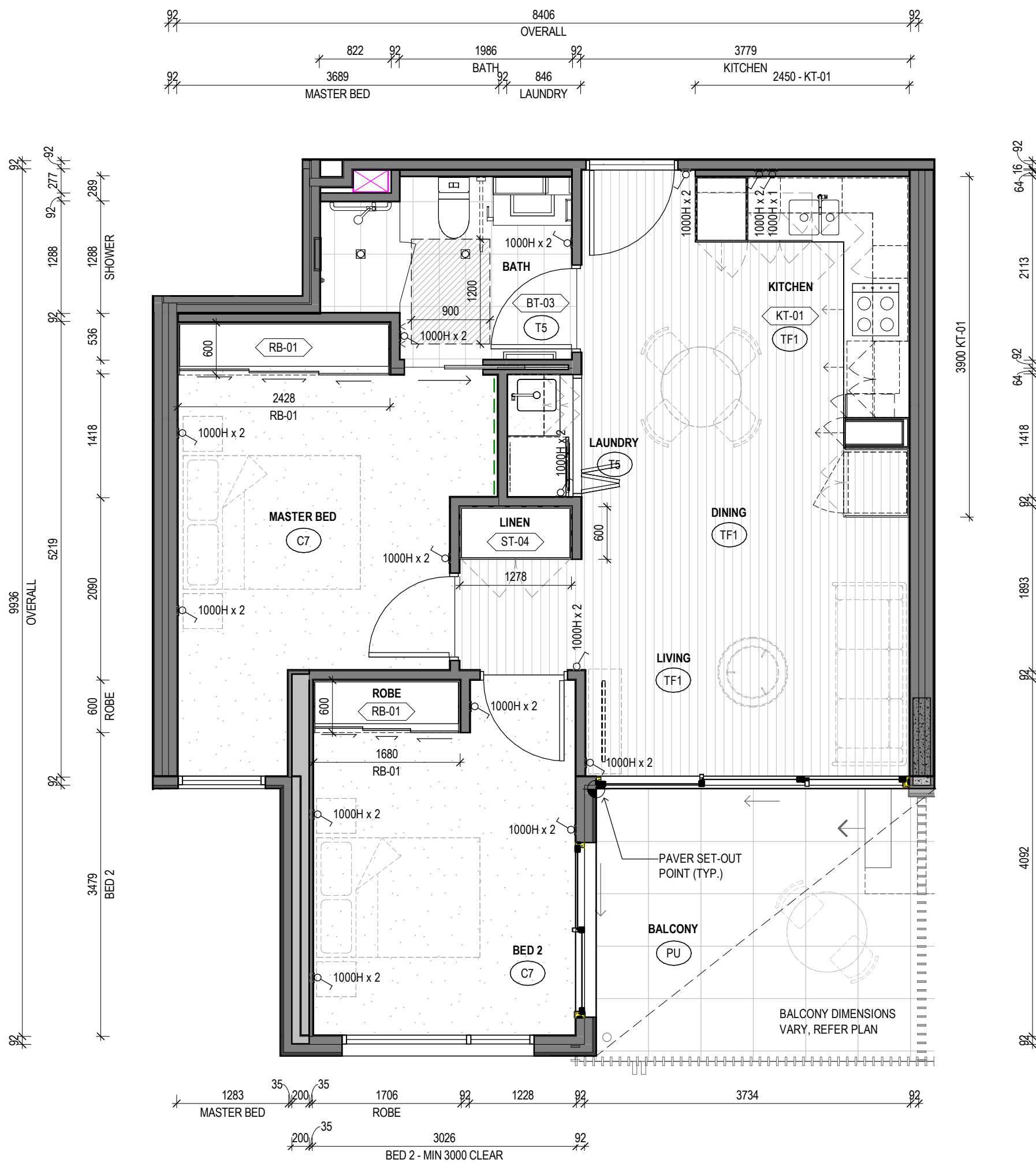
1 ILA Type 3 Scale 1: 50
